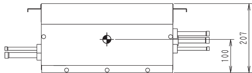
IN CASE OF THE ELECTRICAL BOX ON THE OTHER SIDE OF THE UNIT
