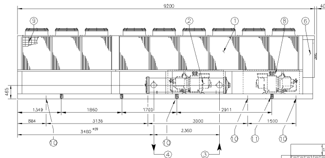
Fan arrangements and minimum clearance requirements
