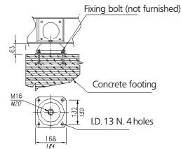
Detail "A" rubber isolator
