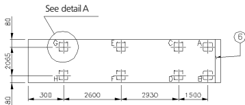
Isolators location
