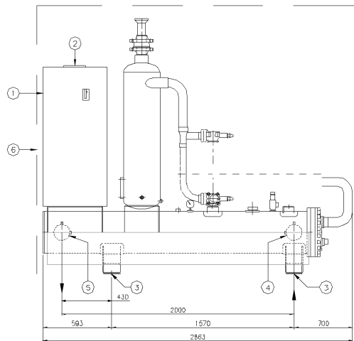
Recommended dimensions
