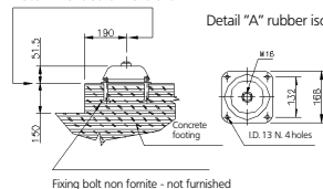
Recommended dimensions
