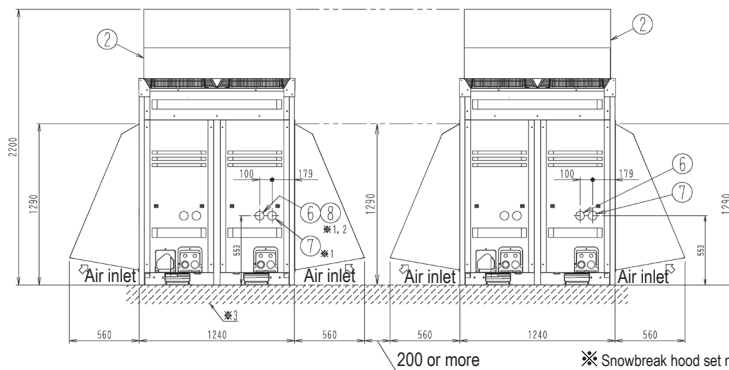
(Master unit)
