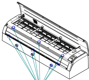
Front grille fixing screws
