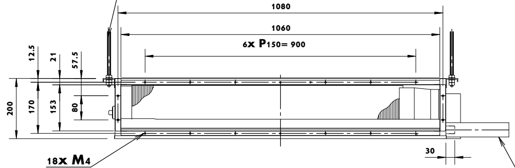
SUSPENSION BOLT 4x M8 ~ M10
