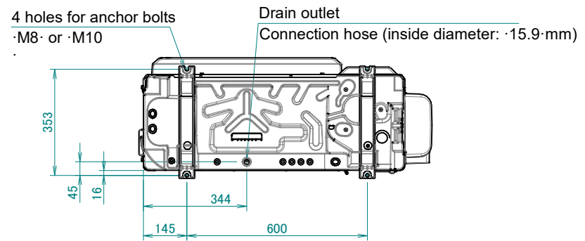
Bottom view
