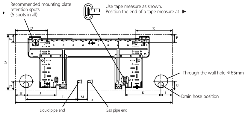
Installation plate ATXN25-35NV1B9
