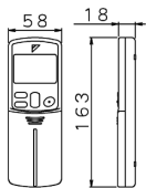
Infrared remote control (ARC433B70)
