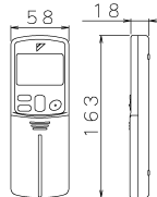
Infrared remote control (ARC433B70)
