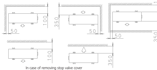
Wall height on air outlet side = less than 1200
