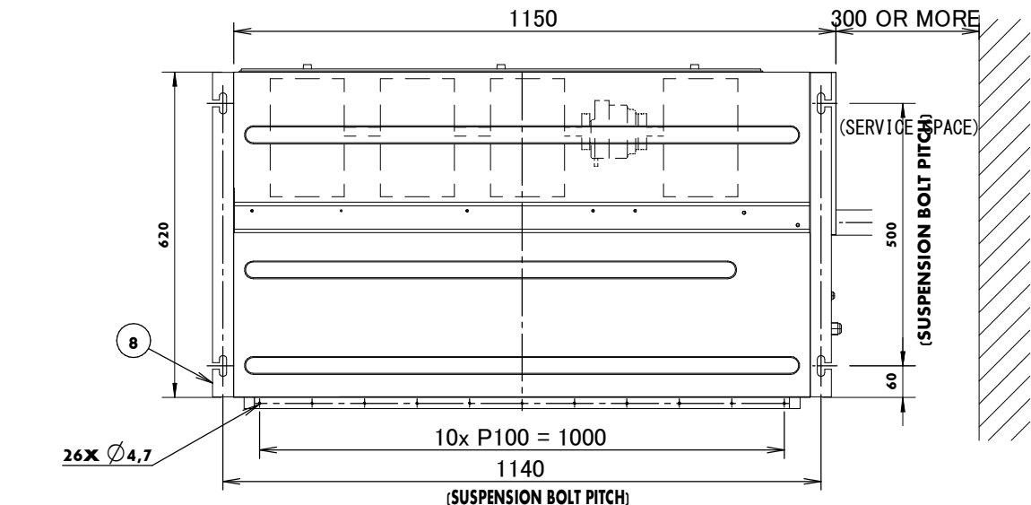
SUSPENSION BOLT 4x M8 ~ M10
