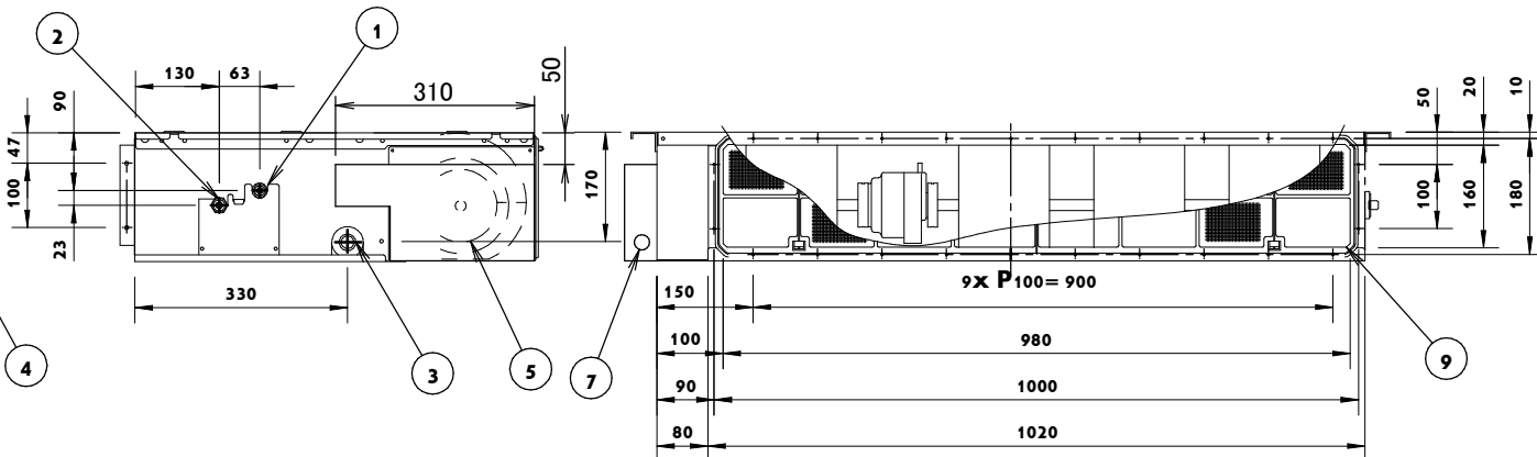
IN CASE OF BACK SUCTION
