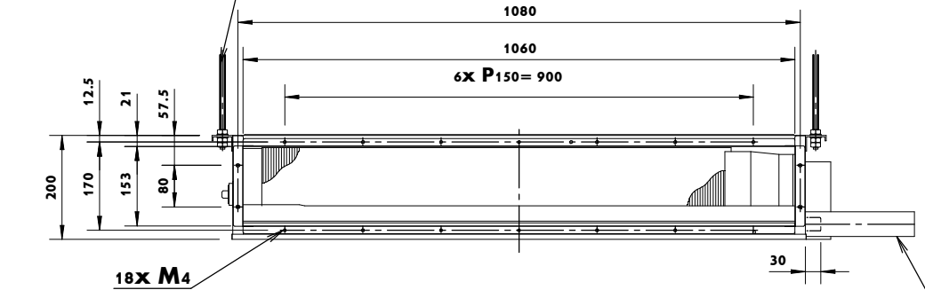
SUSPENSION BOLT 4x M8 ~ M10
