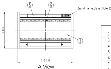
A View
