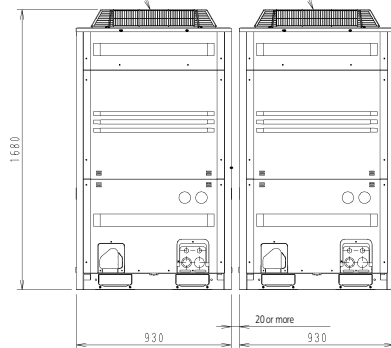
Outdoor unit 1
