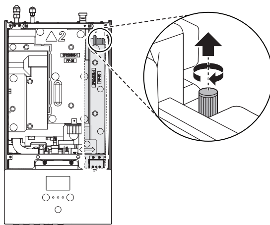
a Valvola Schrader
